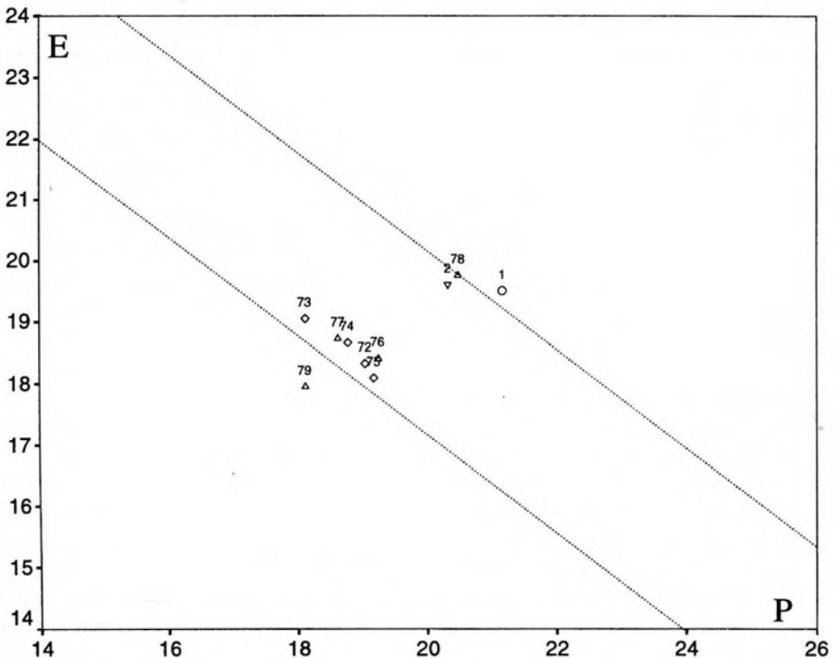
Fig. 16. Pollen dimensions in Anthemis abylaea (○), A. cretica subsp. columnae (▽), A. punctata subsp. punctata (◇), and subsp. kabylica (Δ). E = equatorial inside diameter (μm); P = inside length of polar axis (μm). Dotted lines delimit area of overlap between diploid (bottom left) and tetraploid (top right) OTUs (see Fig. 12).
