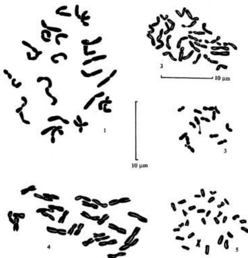
Figs. 1-5. Karyotypes of: 1, Aegilops geniculata , 2n = 28 ; 2, Alopecurus geniculatus , 2n = 28 ; 3, A. gerardii , 2n = 14 ; 4, Dactylis glomerata subsp. glomerata , 2n = 28 ; 5, Dianthus moeniacus , 2n = 30 . — Scale bars = 10 \mu\text{m} .
