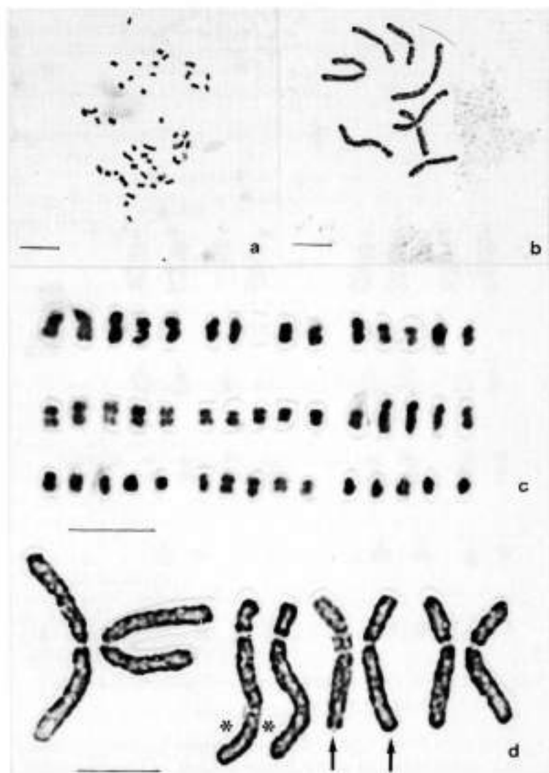
Fig. 2. Mitotic metaphase plates and karyotypes of: a & c, Hyparrhenia hirta (FI-CAM/1), 2n = 45 ; b & d, Bellevalia romana (BA-4166), 2n = 8 . - Asterisks and arrows indicate secondary constrictions and microsatellites respectively. — Scale bar = 10 \mu m.
