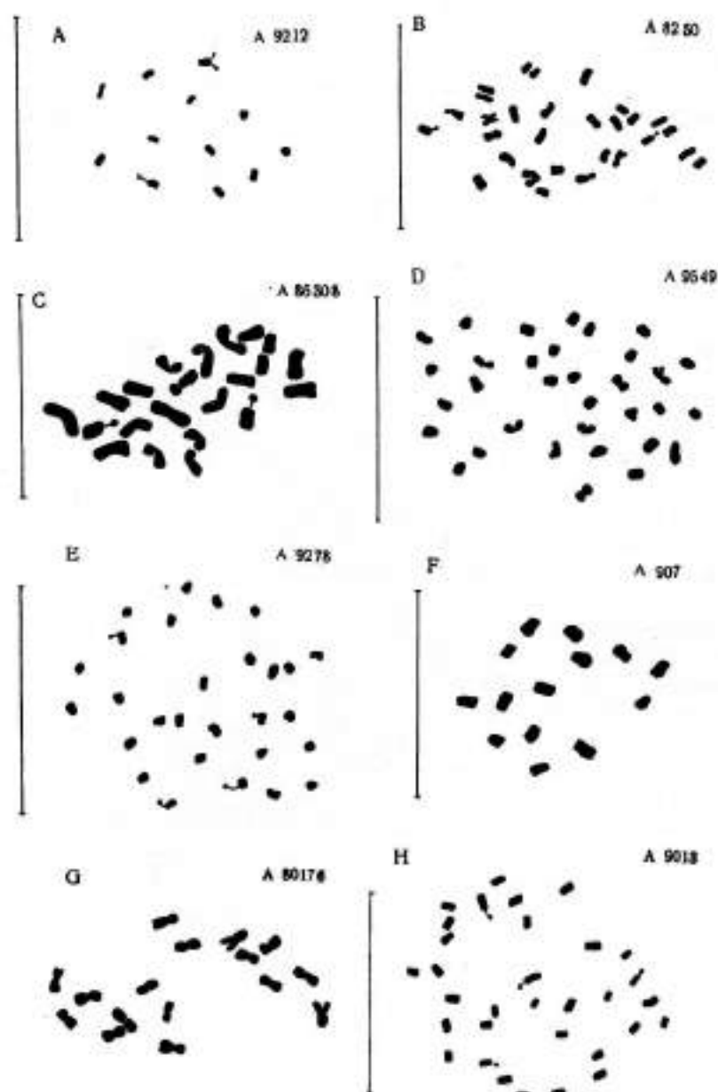
Fig. 5. Mitotic metaphase plates of: A , Hornungia petraea , A9212, 2n = 12 ; B , Limaria rediviva , A8250, 2n = 30 ; C , Iberis sempervirens , A86308, 2n = 22 ; D , I. saxatilis , A9549, 2n = 33 ; E , Isatis praecox , A9278, 2n = 28 ; F , Myagrum perfoliatum , A907, 2n = 14 ; G , Rorippa amphibia , A80176, 2n = 16 ; H , R. sylvestris , A9013, 2n = 32 . — Scale bars = 10 \mu m.
