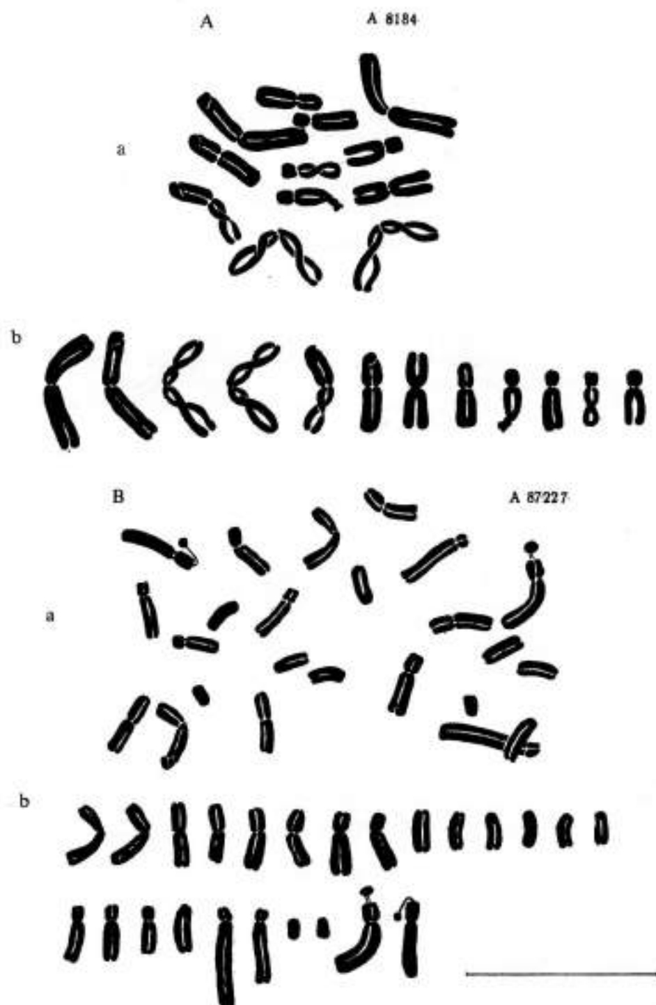
Fig. 2. Karyotypes (a) and karyograms (b) of: A , Hesperis laciniata subsp. laciniata , A8184, 2n = 12 ; B , H. dinarica , A87227, 2n = 24 . — Scale bar = 10 \mu m.
