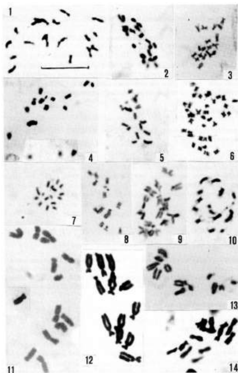
Figs. 1-14. Mitotic metaphase plates of: 1, Bryonia alba , 2n = 20 ; 2, Malabaila dasyantha , 2n = 22 ; 3, Centaurea gulissashvili , 2n = 18 ; 4, Astragalus asterias , 2n = 16 ; 5, Astragalus glycyphyllos , 2n = 16 ; 6, Pseudosophora alopecuroides , 2n = 36 ; 7-8, Sphaerophysa salsula , 2n = 16 ; 9, Lens orientalis , 2n = 14 ; 10, Cicer arietinum , 2n = 16 ; 11, Vicia ervilia , 2n = 14 ; 12, Vicia hyrcanica , 2n = 12 ; 13, Vicia sativa , 2n = 12 ; 14, Lathyrus cicera , 2n = 14 . — Scale bar = 10 \mu\text{m} .
