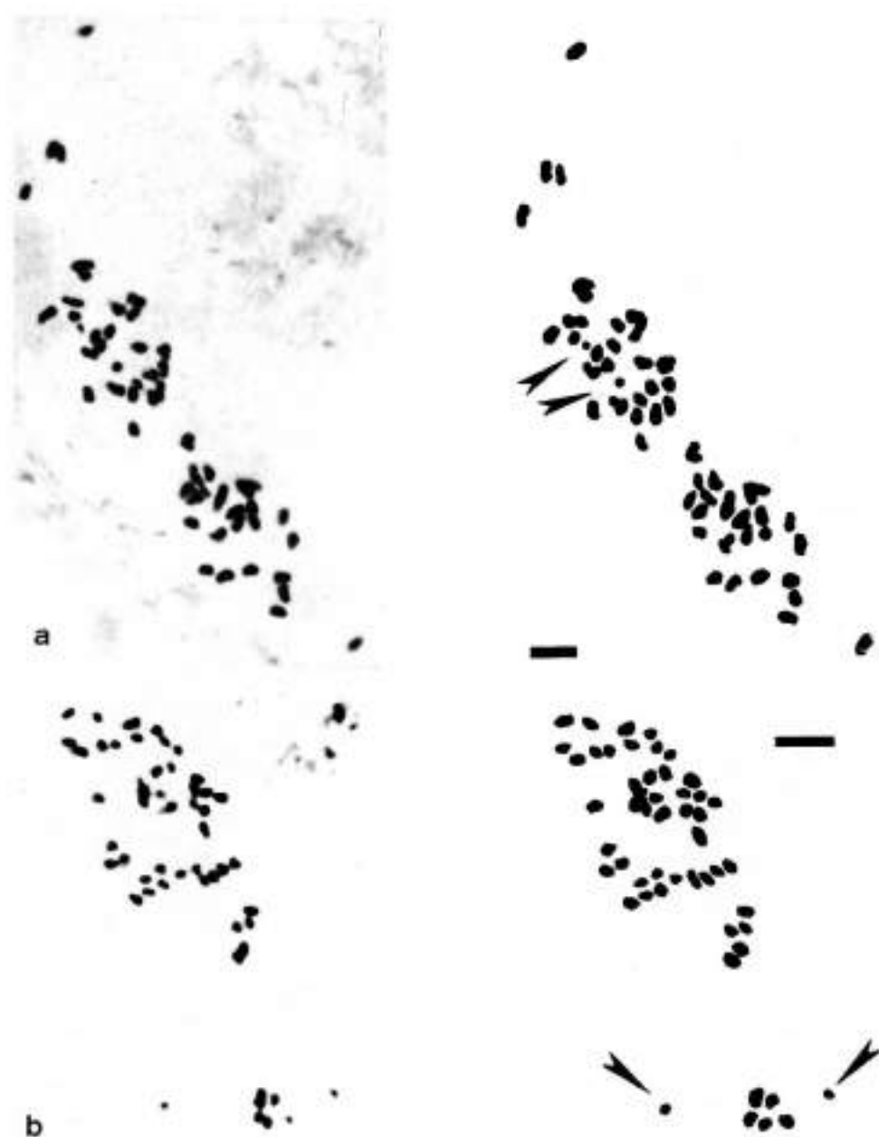
Fig. 1. A photomicrograph and a drawing somatic metaphase plate of: a , Genista acanthoclada - Cesme and b , G. acanthoclada - Taýgetos Oros, 2n = 48 + 2B . Arrows indicate B-chromosomes. — Scale bars = 5 \mu m.
