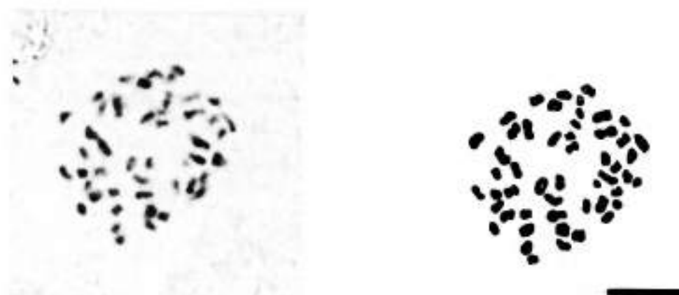
Fig. 2. A photomicrograph and a drawing somatic metaphase plate of Genista aemensis , 2n = 32 . — Scale bar = 5 \mu\text{m} .
