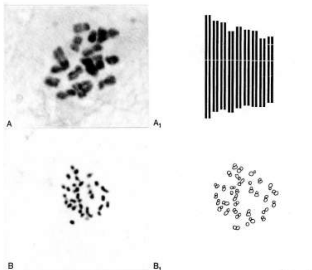
Fig. 2. Mitotic metaphase plates of: A-A 1 , Anthemis hydruntina , 2n = 18, photo and idiogram; B-B 1 , Cirsium carniolicum , 2n = 34, photo and drawing. — Scale bar = 10µm.
