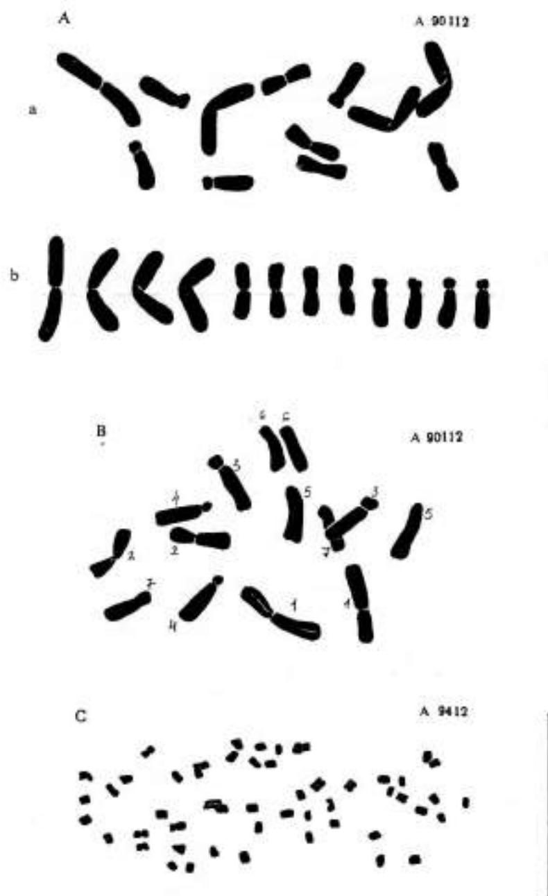
Fig. 3. Karyotypes (a) and karyogram (b) of: A, Hesperis sylvestris var. velenovskii , A90112, 2n = 12 ; B, Hesperis sylvestris var. velenovskii , A90112, 2n = 14 ; C, Erophyla verna , A9412, 2n = 52 . — Scale bar = 10 \mu\text{m} .
