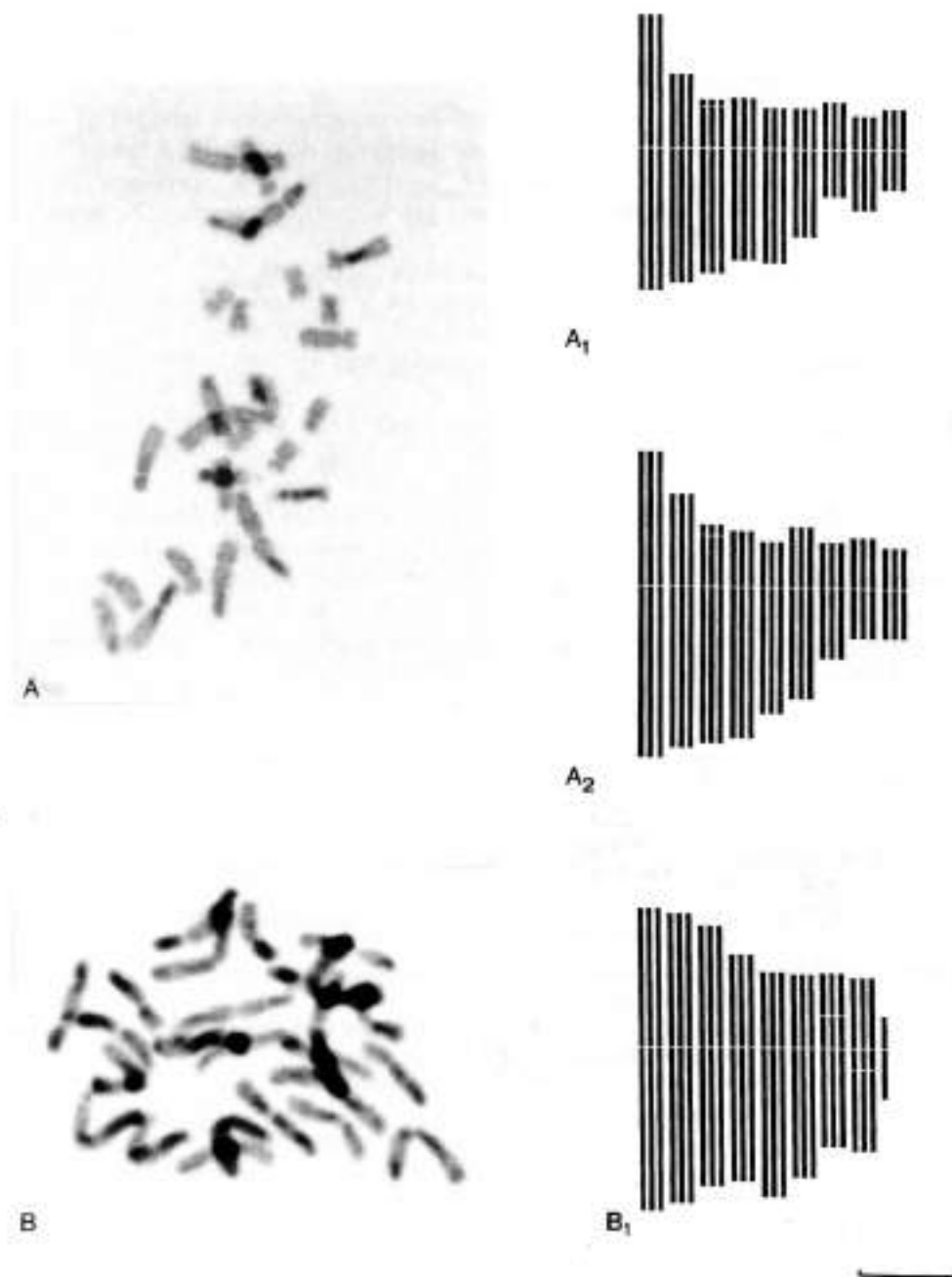
Fig. 3. Mitotic metaphase plates of: A-A 1 -A 2 , Ornithogalum umbellatum , 2n = 27 , photo and idiograms; B-B 1 , Allium commutatum , 2n = 24 + 1B , photo and idiogram. — Scale bar = 10 μm.
