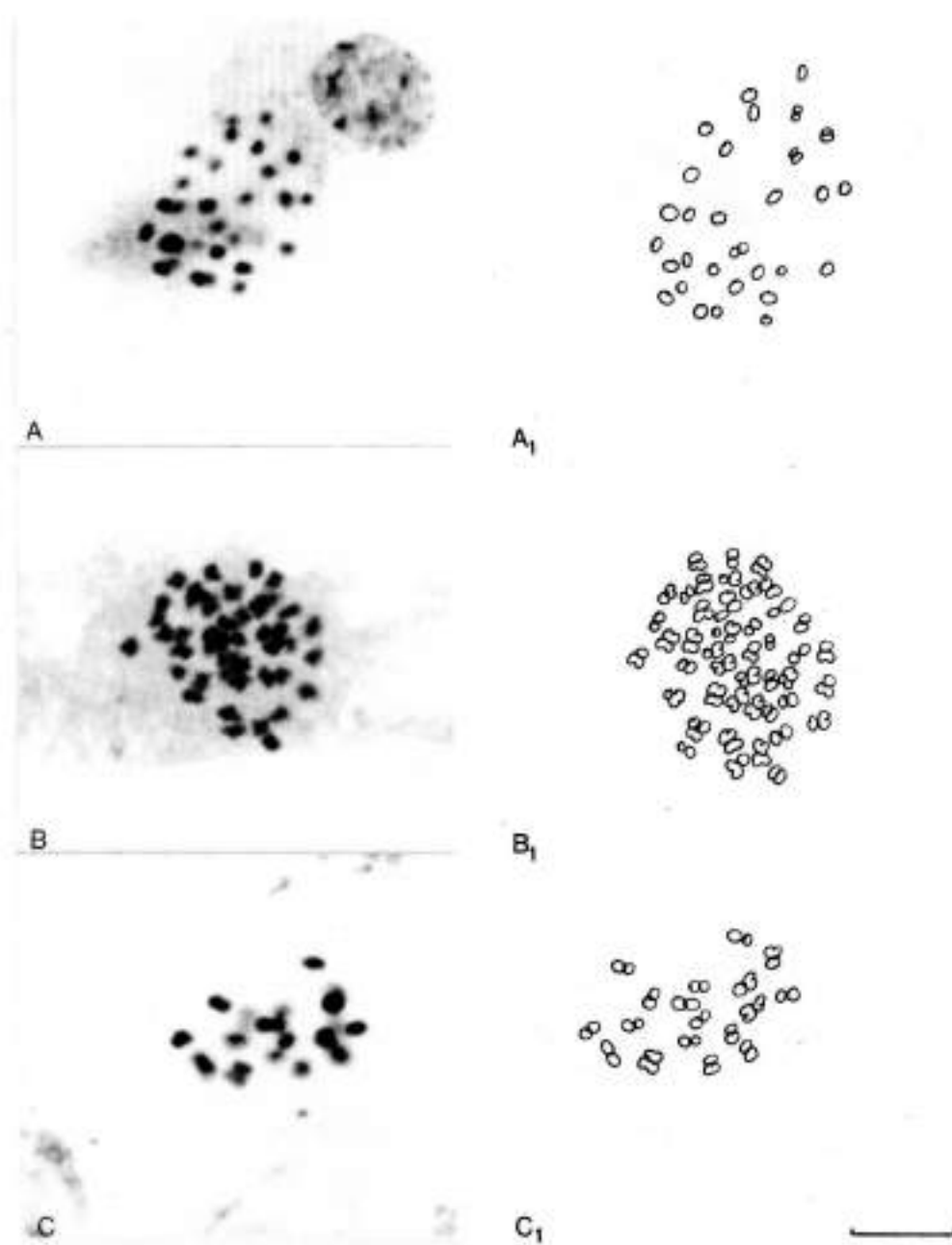
Fig. 1. Mitotic metaphase plates, photos and drawings, of: A-A 1 , Dianthus jupigicum , 2n = 30 ; B-B 1 , Opuntia compressa , 2n = 44 ; C-C 1 , Wulfenia carinthiaca , 2n = 18 . — Scale bar = 10\mu\text{m} .
