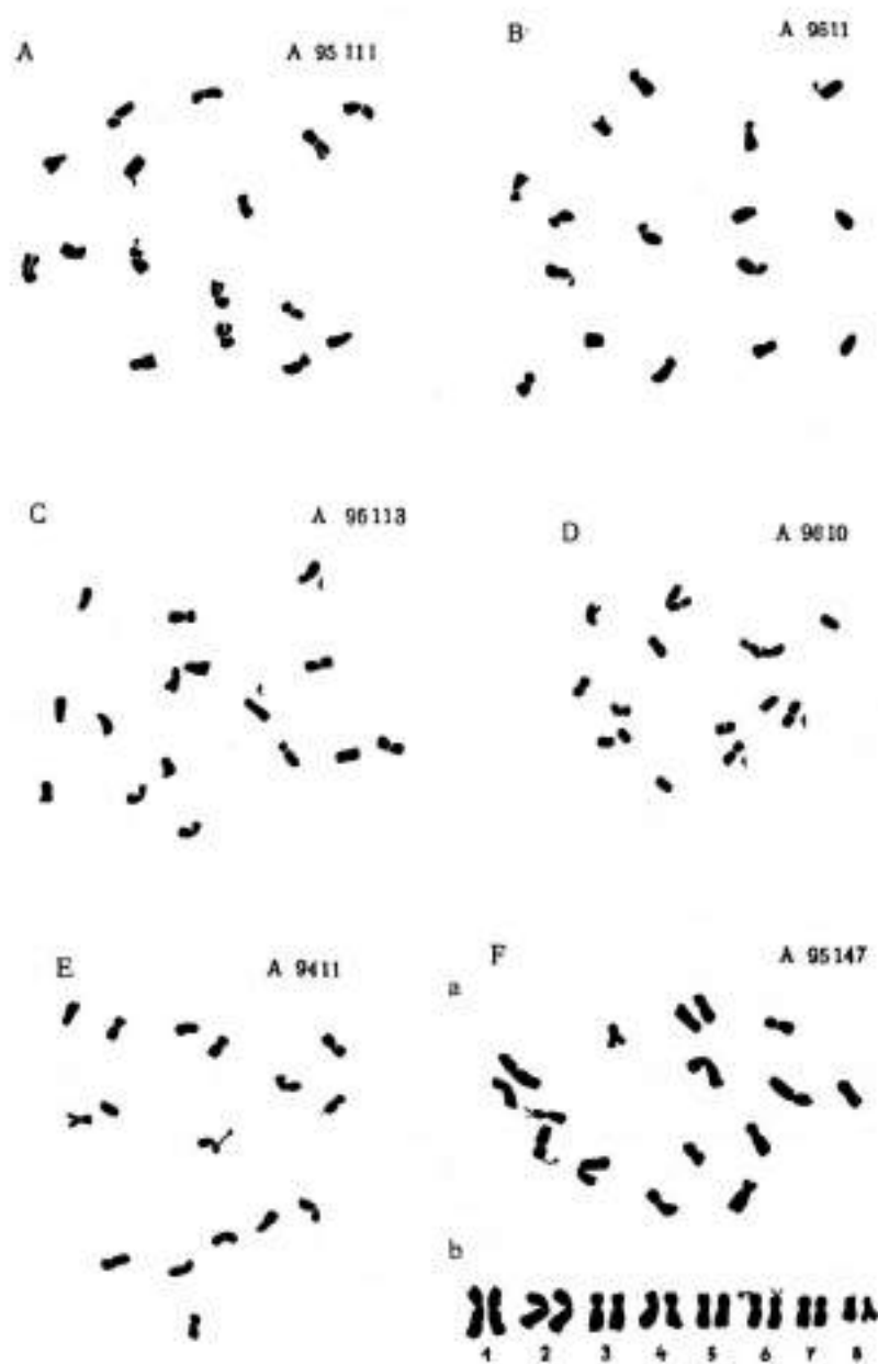
Fig. 1. Mitotic metaphase plates of: A, B, Cardamine acris , 2n = 16 ; C, D, C. amara subsp. amara , 2n = 16 ; E, C. matthioli , 2n = 16 ; F, karyotype (a) and karyogram (b) of C. rivularis , 2n = 16 . — Scale bar = 10 \mu m.
