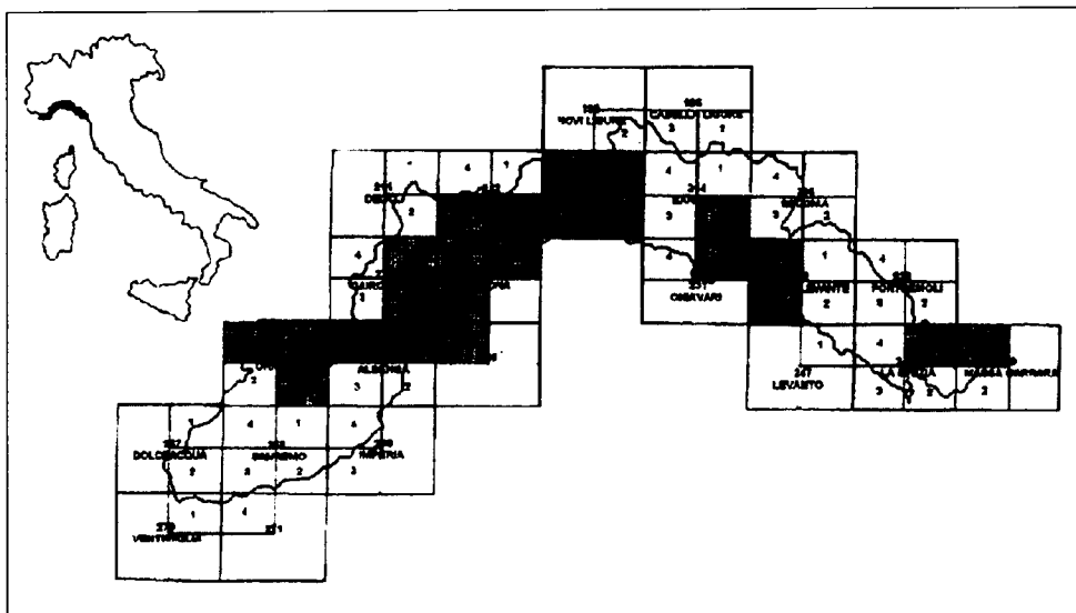
Fig.1: Italy and Liguria (upper left corner) and localization of studied areas (shaded rectangles) within Liguria. The numbers in the map refer to the "Regional Technical Cartography" of Liguria. Each rectangular area is approximately 130 Km 2 .
