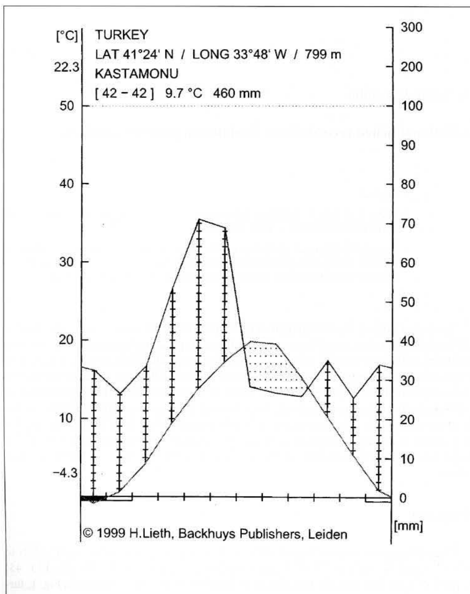
Fig. 1. Climate diagram of Kastamonu representing the survey area (from Lieth et al. 1999).
